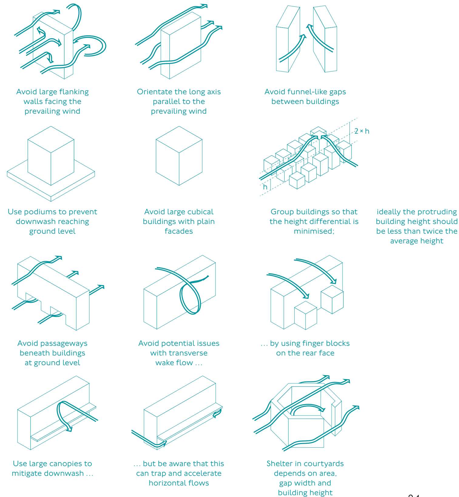
Figure 0.2: Example of wind flow around buildings and how to minimise the impact
