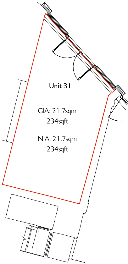
Ground Floor @ 1:100
